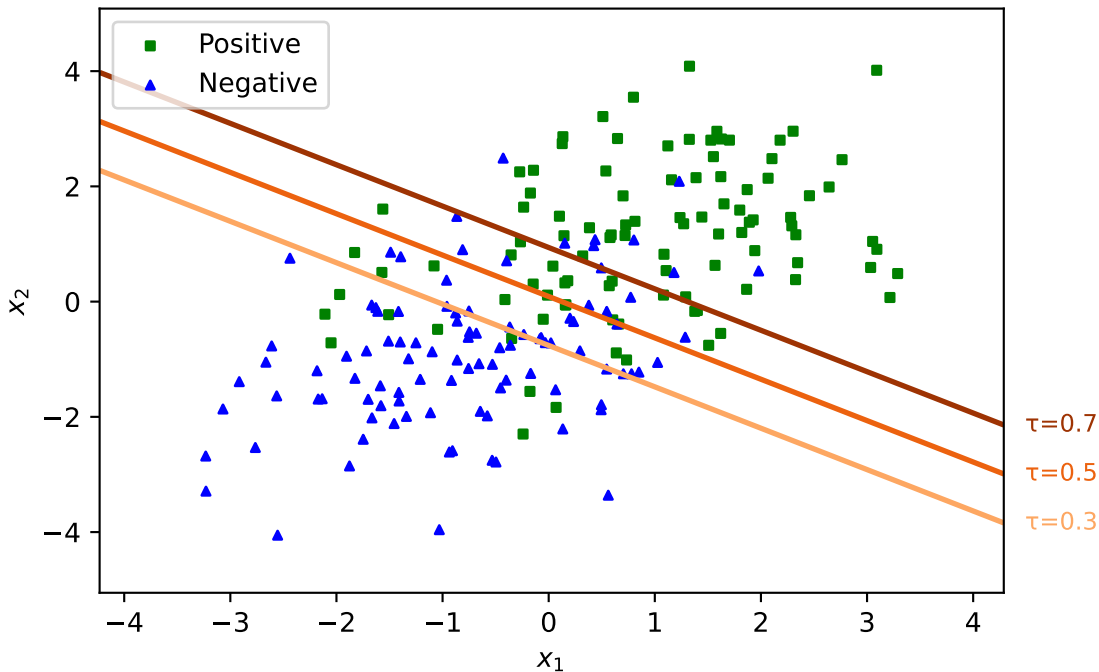
Decision Boundaries with Varying Thresholds
